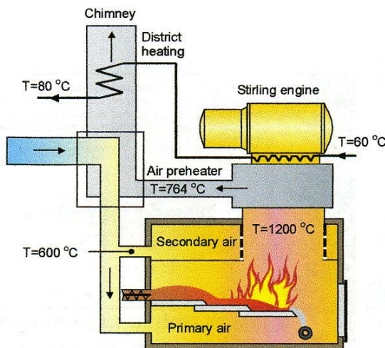
Schema of a biomass CHP system based on a Stirling engine (Source: BIOS Bioenergy Systems, Austria 2003)
